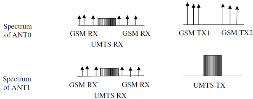
Figure 8 Typical Spectrum of Passive Type 2 combiner (at the antenna port)
