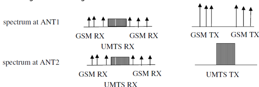
Figure 2 Typical Spectrum of Active Type 1 Combiner
