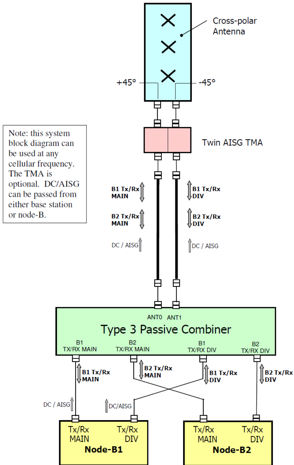
Figure 11 Passive Type 3 Combiner System Block Diagram
