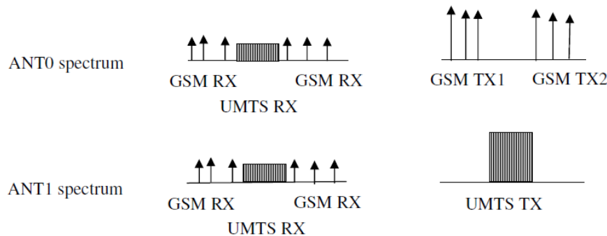
Figure 6 Typical Spectrum of Active Type 2 Combiner (at antenna ports)
