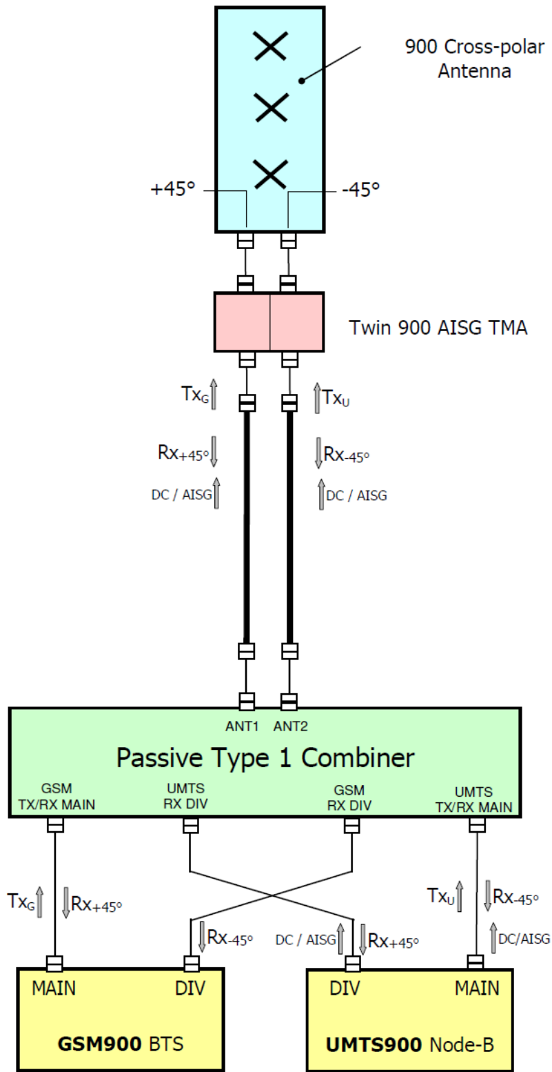
Figure 5 Passive Type 1 Combiner - System Block Diagram
